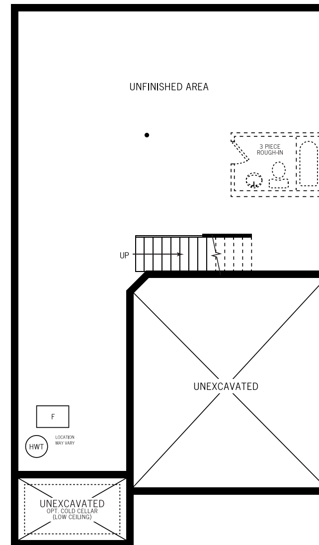
Unfinished Basement ELEVATION A & C
