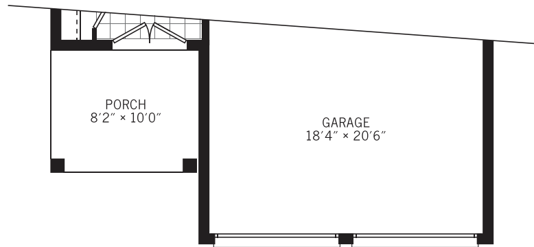
Ground Floor ELEVATION B
